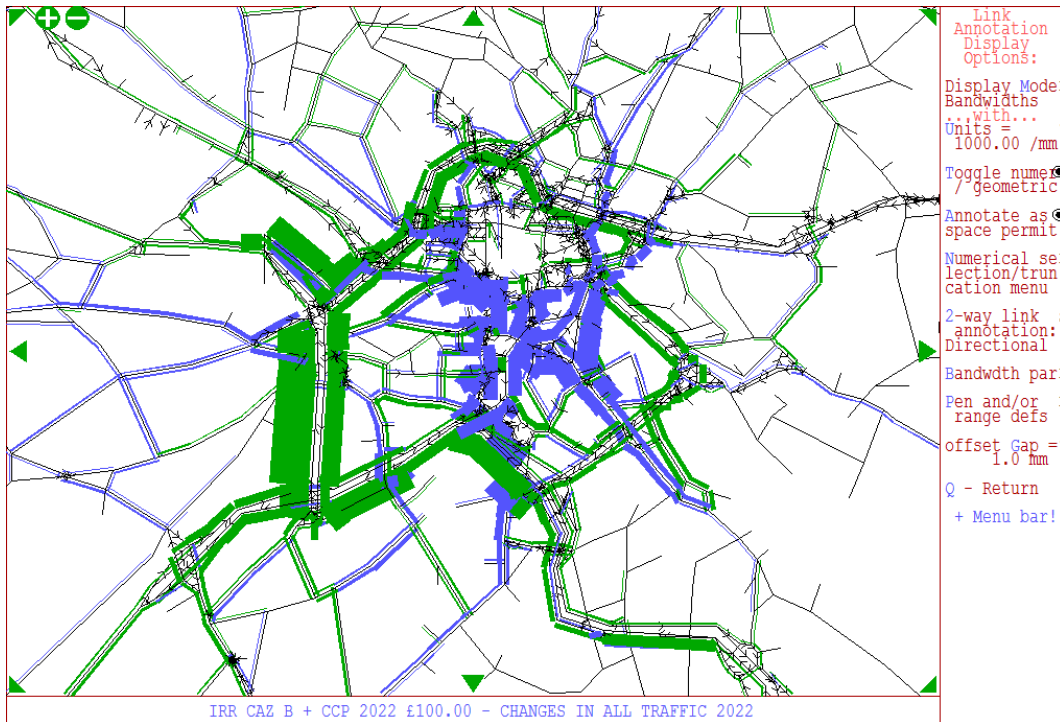
Figure 13 – Total Traffic Changes (12 hour pcus) 2022
